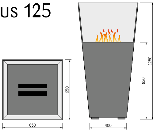
Venus 125 in Bar
